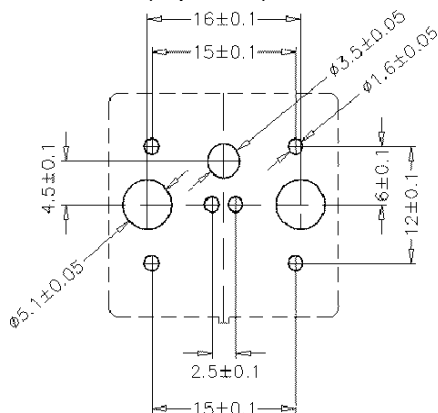
for use with socket pins (top view)
