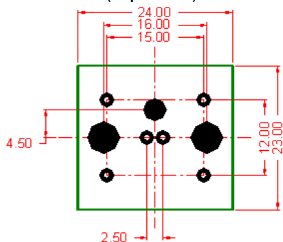
Direct PCB Mount (top view)
